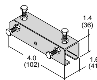
NOTCHED COUPLER/HANGER #C35-CP-01 Weight = 1.0 lbs COUPLER/HANGER BRACKET #C35-CP-02 Weight = 1.25 lbs
