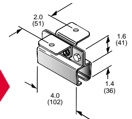
NOTCHED COUPLER/HANGER #C35-CP-01 Weight = 1.0 lbs COUPLER/HANGER BRACKET #C35-CP-02 Weight = 1.25 lbs
