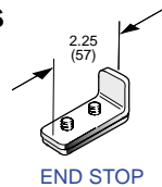
END STOP #WS30-ES Weight = 0.3 lbs
