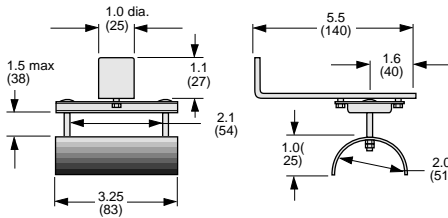
FLAT CABLE END CLAMP #C35-FE-02 Trolley Weight = 1.46 lbs
