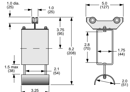
FLAT CABLE TOW TROLLEY #C35-FT-52 Trolley Weight = 2.28 lbs
