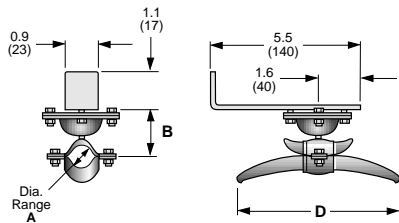
ROUND CABLE END CLIP
